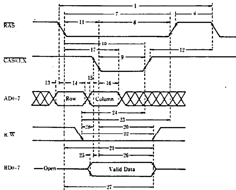
VRAM write cycle (early write)
