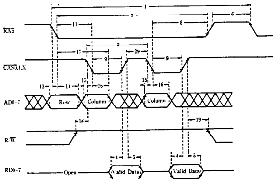
VRAM page mode cycle
