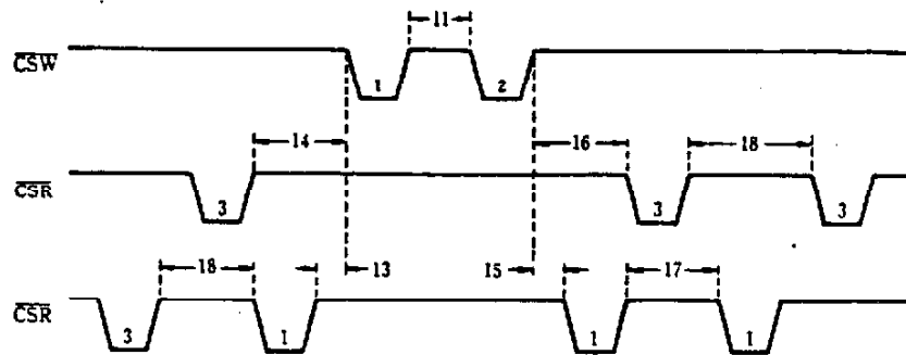
CPU-MSX-VIDEO read cycle interface
