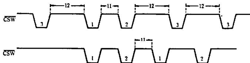
MSX-VIDEO register read timing
