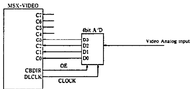
Digitize Block Diagram (GRAPHIC 4 mode)
