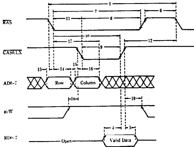
VRAM read cycle
