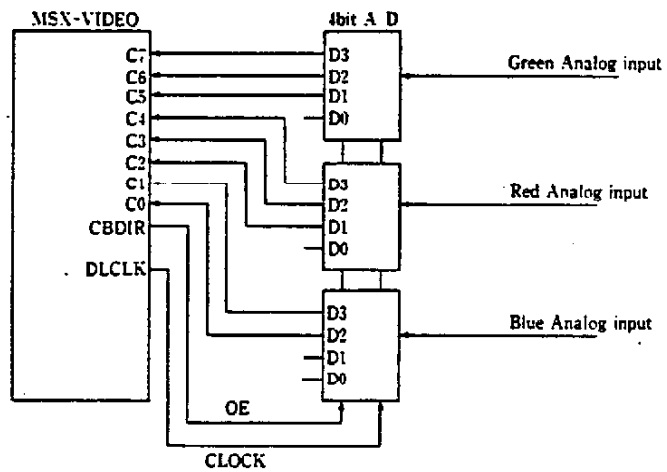
Digitize Block Diagram (GRAPHIC 4 mode)
