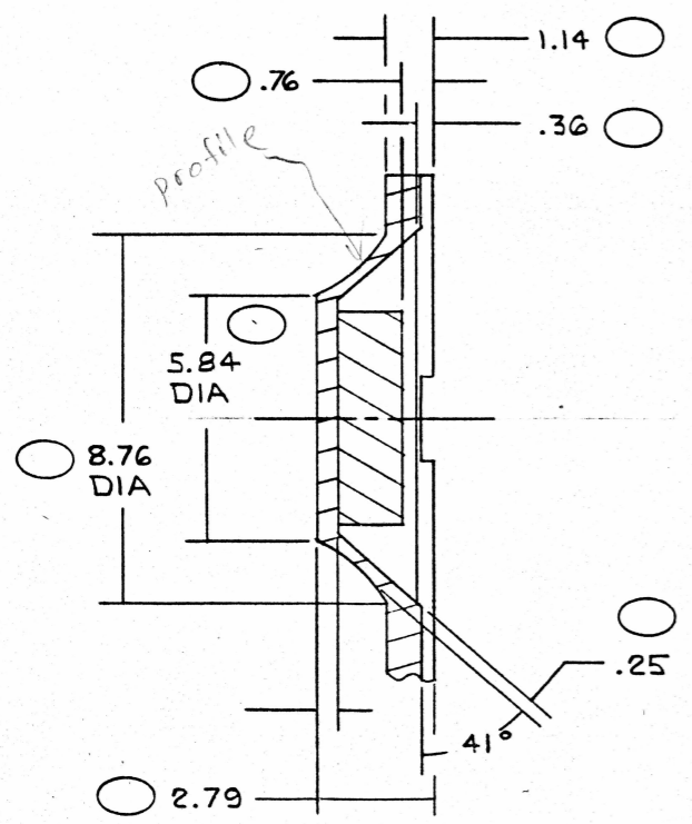
SECTION A-A SCALE 10 X
