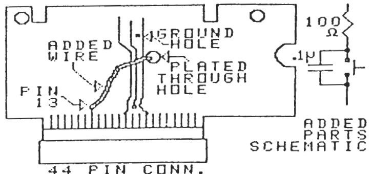
BOTTOM VIEW OF SPEECH SYNTHESIZER BOARD
